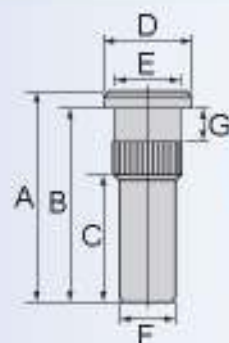
Wheel Bolt - 10.9 Strength
