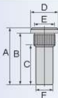
Wheel Bolt - 10.9 Strength
