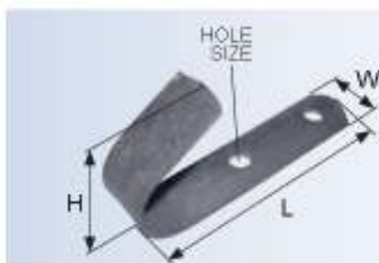
Lightweight Rope Hook - 2 Hole
