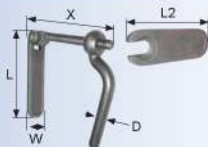
Heavy Duty Ramp Fastener (5/8" ACME Threaded)
